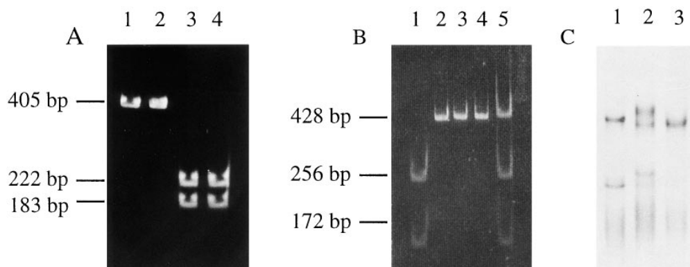
Figure 4.—PCR-RFLP and SSCP analysis used to distinguish the four porcine MC1R variants. (A) AccII RFLP of PCR products obtained with primer pair EP1G1/EP1G3 reflecting sequence polymorphism at codon 240. The test distinguished DNA amplified from Duroc ( MC1R *4/4, lane 1) and Meishan ( MC1R *2/2, lane 2) from that of wild boar ( MC1R *1/1, lane 3) and Large White ( MC1R *3/3,
